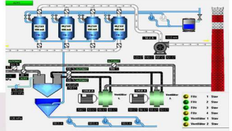
SCADA SYSTEM
